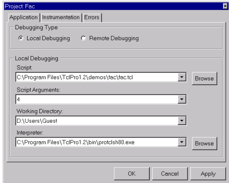
Figure 4 The Project Application Settings Tab, Local Debugging
