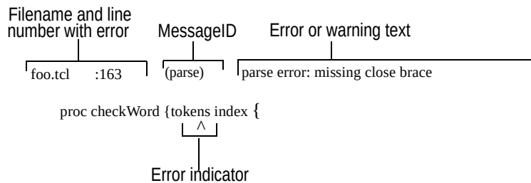
Figure 20 Anatomy of a TclPro Checker Message
