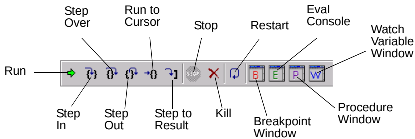
Figure 2 TclPro Debugger Tool Bar
