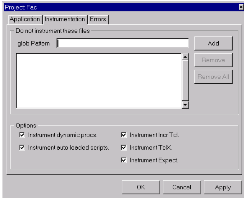
Figure 6 The Project Instrumentation Settings Tab
