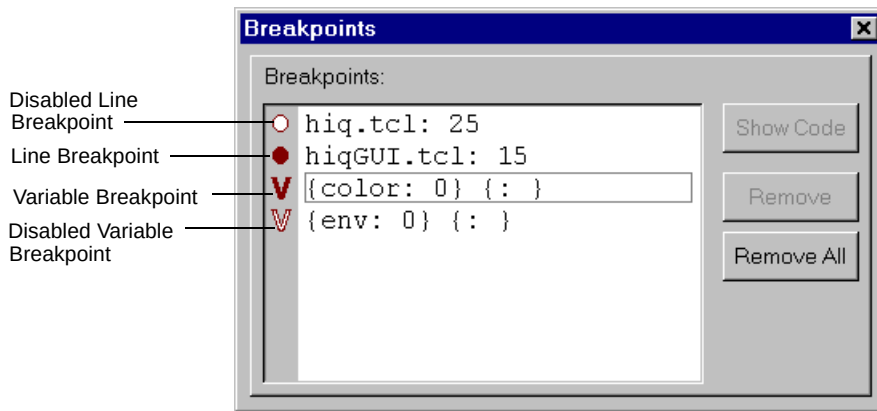
Figure 9 The Breakpoints Window
