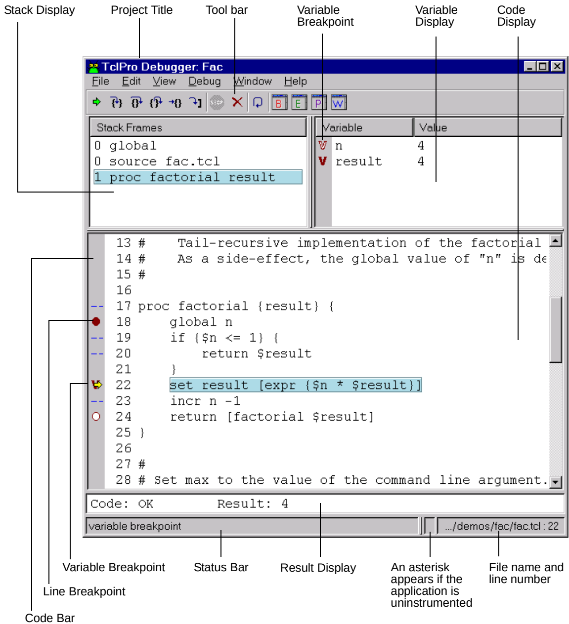
Figure 1 TclPro Debugger Main Window
